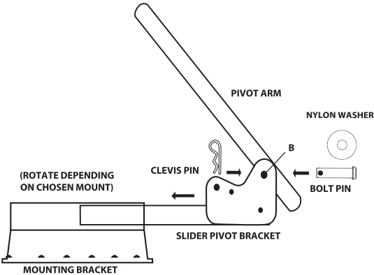
ILLUSTRATION 5 ASSEMBLY OF SLIDER ARM TO PIVOT ARM SIDE VIEW
