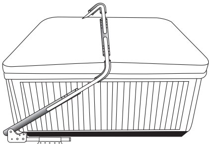
DECK OR FLOOR MOUNT ONLY - SIDE VIEW
