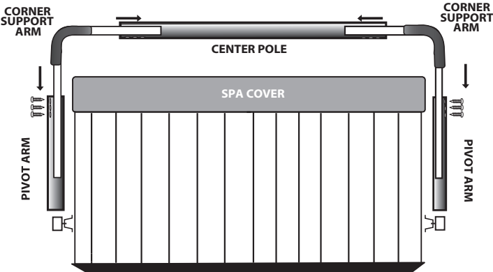
ILLUSTRATION 4 ASSEMBLY OF CORNER ARMS TO PIVOT ARMS - FRONT VIEW
